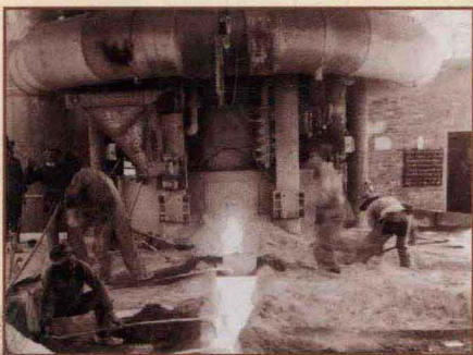
71立方米高炉出第一炉铁水 The first ladle of pig iron produced by 71-cubic-meter blast furnace
