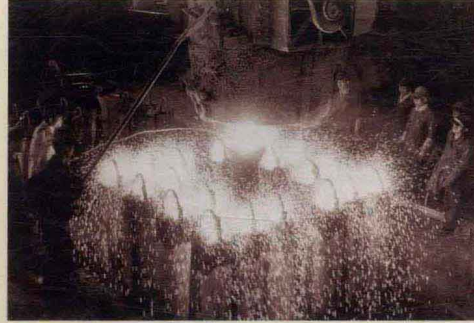
浇铸钢锭 A steel ingot being cast
