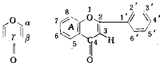
γ-pyrone
