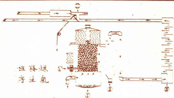
Diagram Shows the Process of Gasifying.
