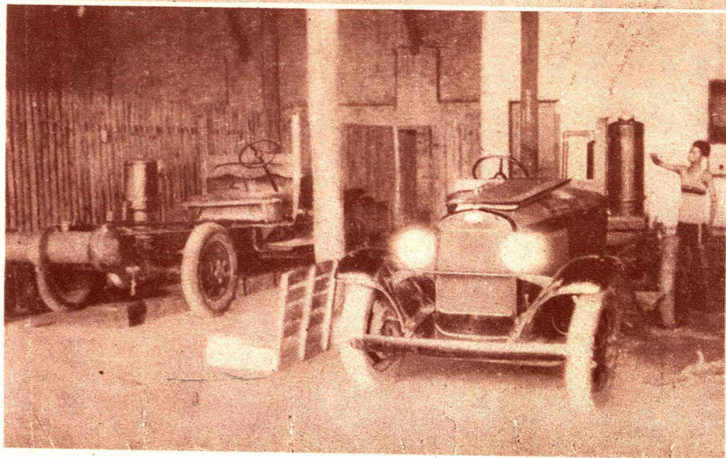
← 一理之構，不位置雖式集者，明為左中裝正車兩輛 。則原造但同置之裝；成為右式仲者，造在，汽中 The Two Different Types of Charcoal-gas Automobiles Operating on the same Principle.
