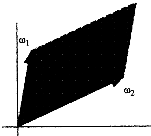
An Oriented Basis for the Lattice \Lambda
