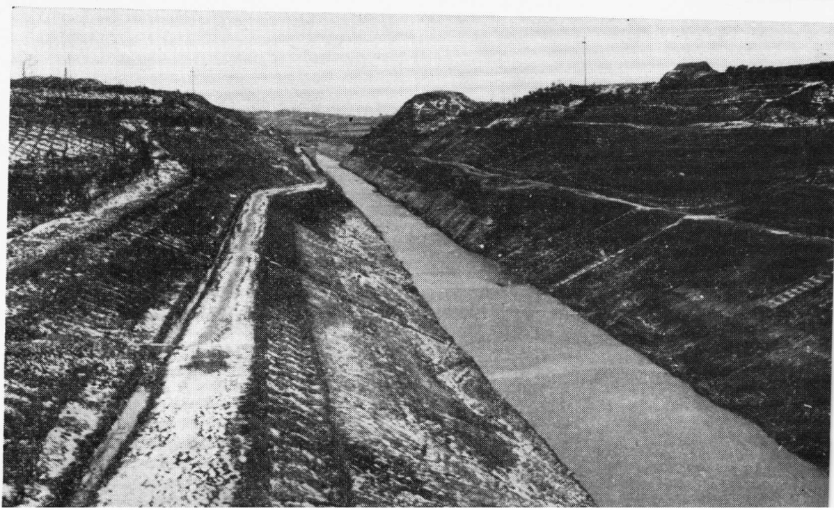
New canal, Shaoshan, Hunan.
