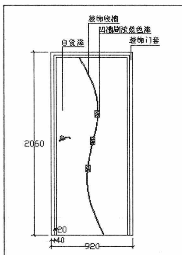
绘制门及门套·····100
