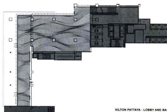
HILTON PATTAYA - LOBBY AND BAR CEILING FABRIC INSTALLATION PLAN
