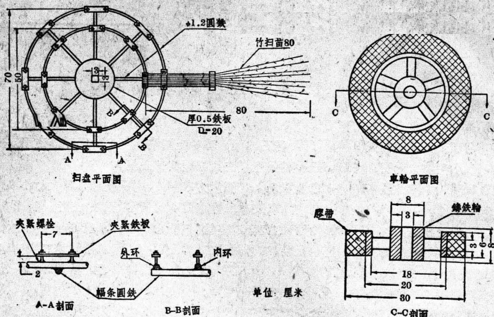
圆盘式扫砂車②
