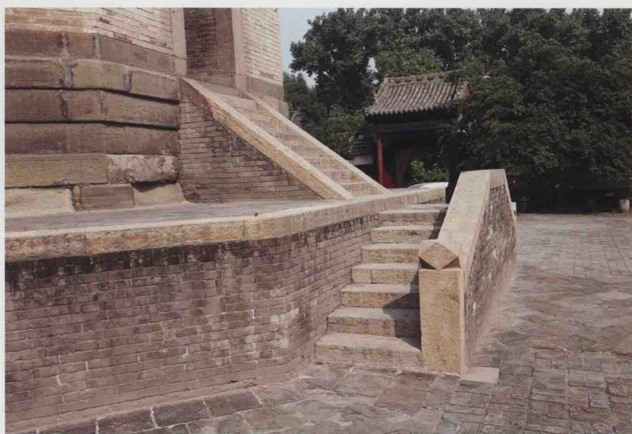
晋祠浮屠院舍利生生塔台阶
