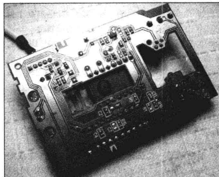
(从电路板后面焊上微动开关)
