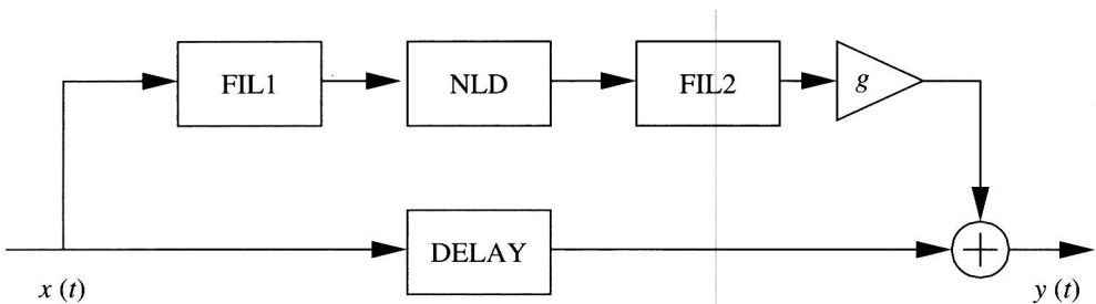
Figure I.2 General BWE framework, also shown as high-frequency BWE structure in Fig. 5.2. Similar structures are shown for low-frequency psychoacoustic BWE as Fig. 2.4 and for low-frequency physical BWE as Fig. 3.1
