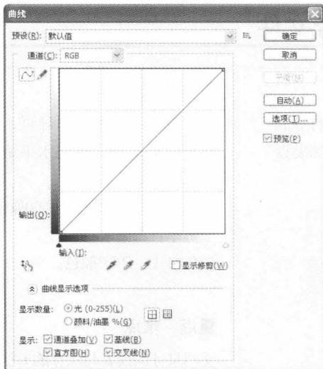
图1-24 “曲线”对话框
