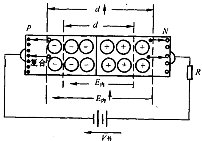
图1-6 PN结反向加压
