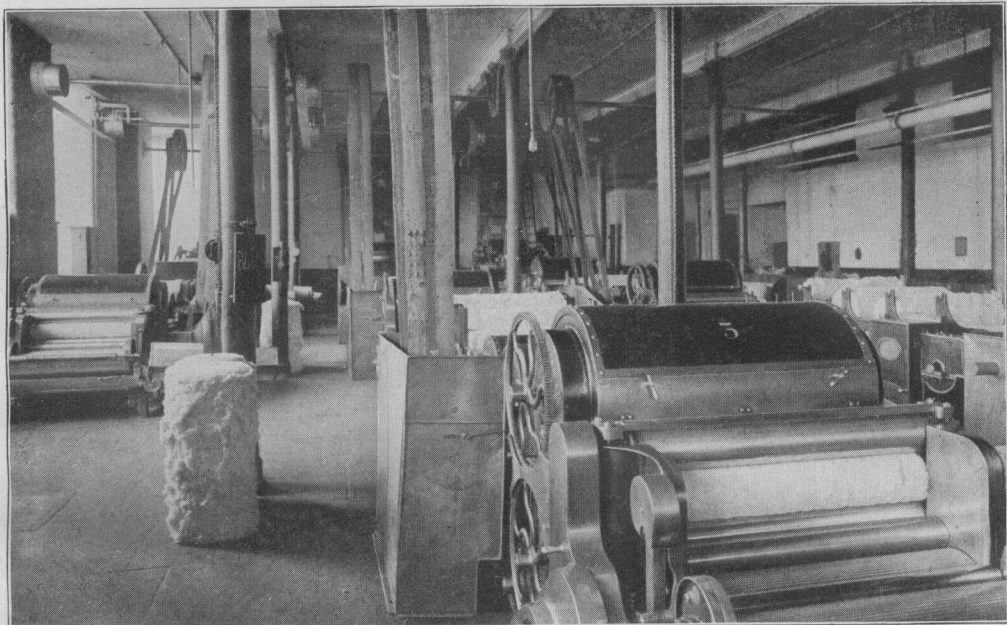
Fig. 10.—Blowing Room.
