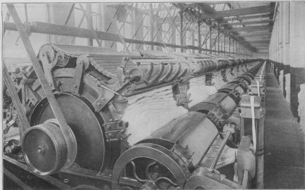
Fig. 11.—Carding Room.
