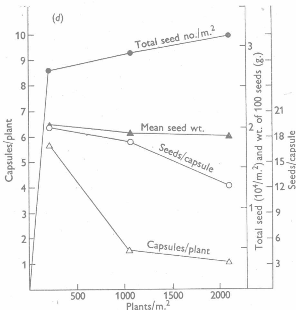
Fig. 1 continued. (c) Sunflower ( Helianthus annuus ). After Clements, Weaver & Hanson (1929). (There is some indication in Clements' data that a degree of self-thinning had occurred at high densities and so the number of plants per unit area was probably not directly proportionate to density of seeds sown.) (d) Corncockle ( Agrostemma githago ). Original data.
