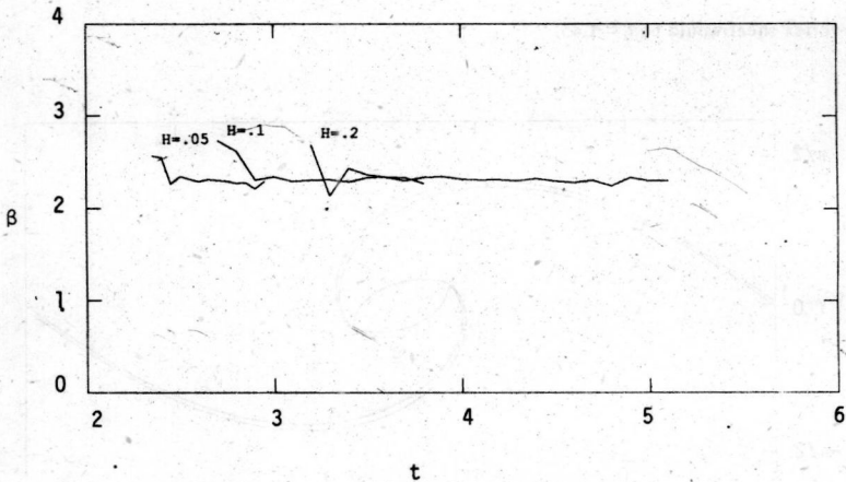
Figure 2. \beta as a function of time for various mean thicknesses H .
