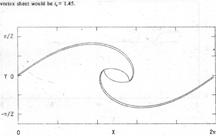
Figure 1. The location of the vortex layer of mean thickness H = 0.1 at time t = 4.0 . The initial amplitude a = 0.5 .
