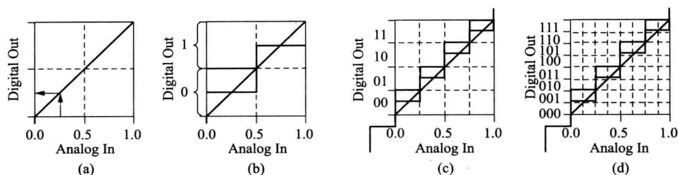
Fig. 1-2 Quantize a ramp signal with a 1-bit quantizer
