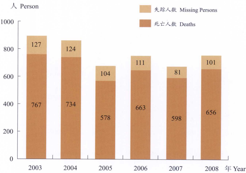
图16 2003~2008年地质灾害造成人员死亡和失踪情况 Fig.16 Deaths and missing persons caused by geological hazards in 2003~2008
