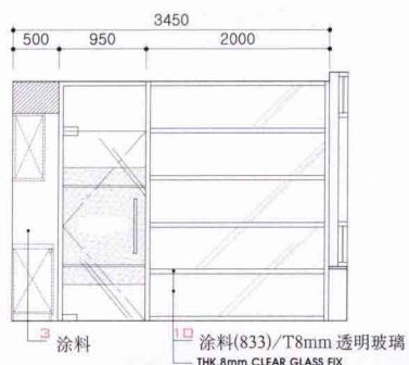
手术室立视图 D/elevation D(operation room)
