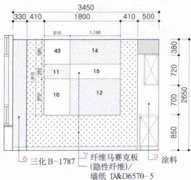
手术室立视图 B/elevation B(operation room)
