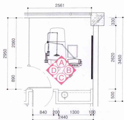
手术室楼平面图 / floor plan(operation room)
