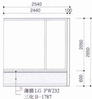
手术室立视图 A/elevation A(operation room)
