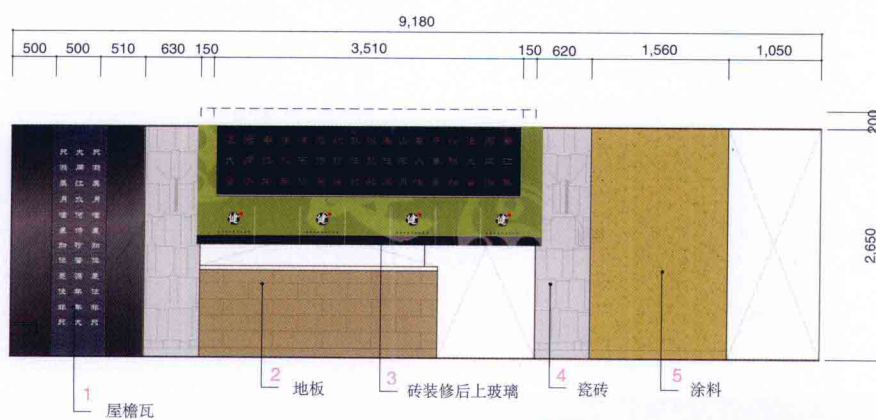
厨房立视图 / elevation(kitchen)
