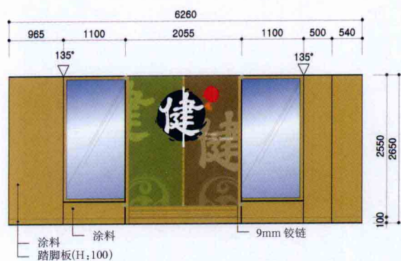
柜台墙立视图/elevation(counter wall)
