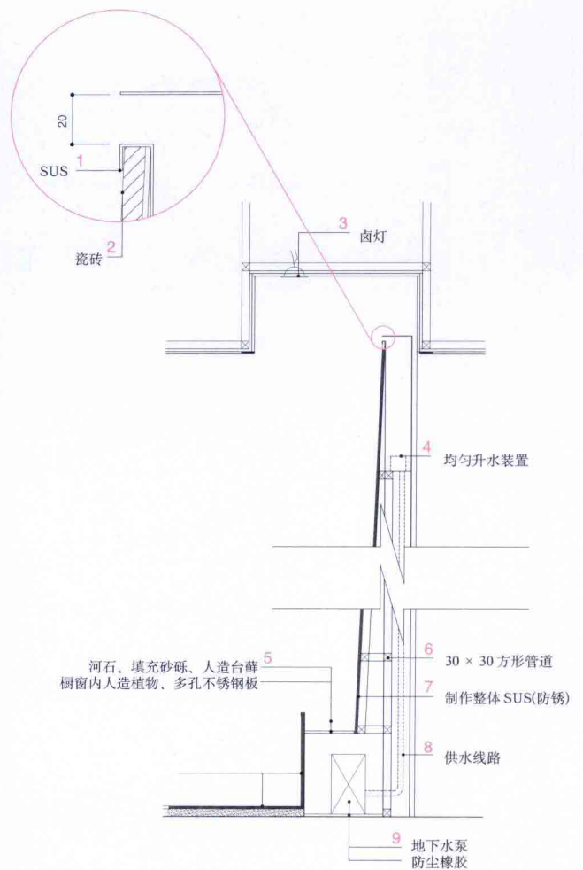
喷泉墙详图 / wall detail (wall fountain)
