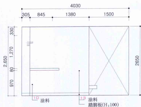
柜台立视图/elevation(counter)
