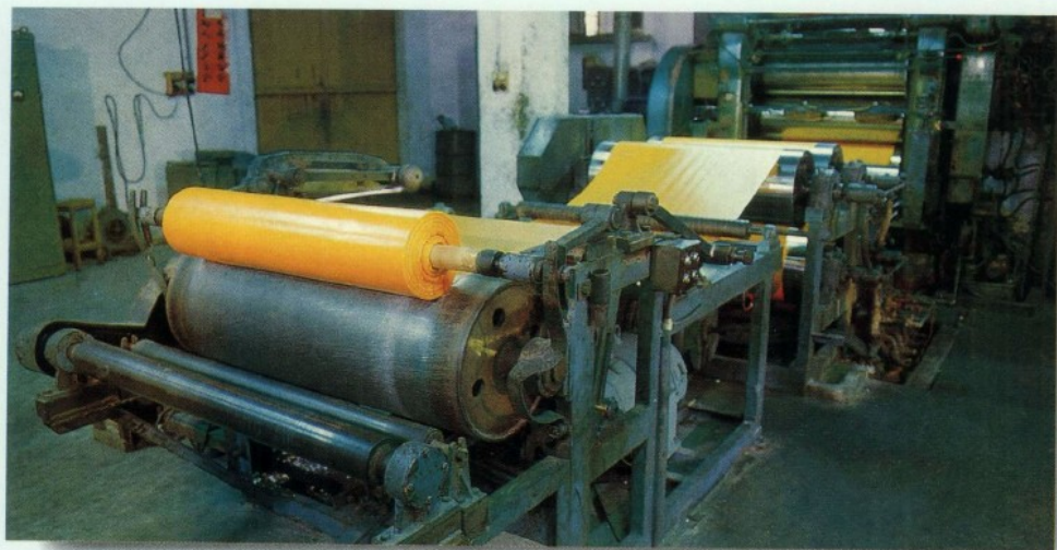
▶ 汕头塑料二厂压延薄膜生产线
