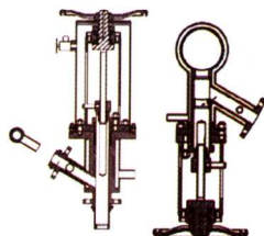
排放阀 Drain Valve
