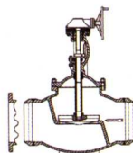
大口径波纹管截止阀 Large Port Bellows Globe Valve
