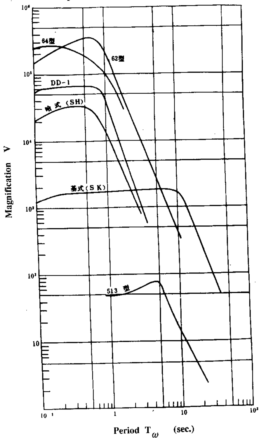
仪器放大倍率曲线 Response Curves of Instruments
