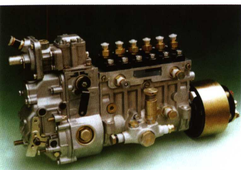
PW 泵
