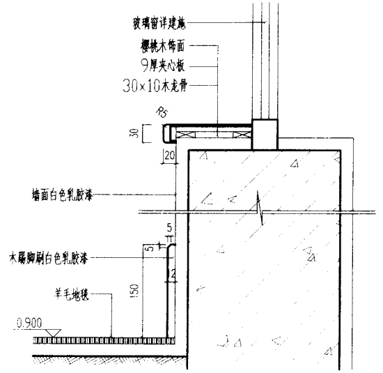
(C) 窗台大样图
