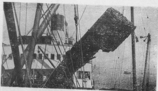
34-Ton Locomotive Boiler For Canton-Hankow Railway Being Discharged From M. V. Memnon at Hongkong
