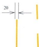
禁驶区标线尺寸
