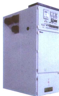
KYN28B-12(Z)型铠装移开式交流金属封闭开关设备
