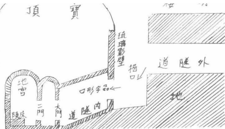
繪會員委陵東收接。◁圖宮地陵禧慈禧▷ Cross sectional view of the tomb for Empress.
