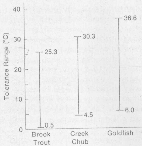
Figure 2-1 Different species have different ranges of tolerance. The goldfish is able to live in warmer waters than the brook trout but does not tolerate cold temperatures as well as the brook trout. (From J. R. Brett, "Some principles in the thermal requirements of fishes," Quarterly Review of Biology , 31:75, 1956.)
