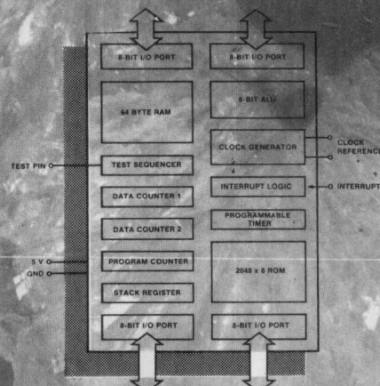
F3870 MicroMachine 2
