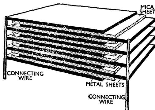
FIG. 3. Electric condenser
