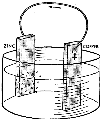
FIG. 4. Simple electric cell
