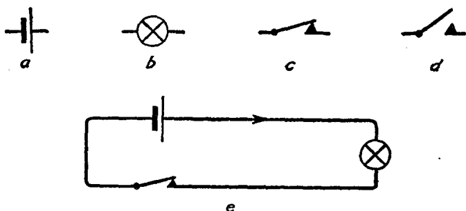
FIG. 7. Symbols for an electric circuit. (a) Battery. (b) Bulb or lamp. (c) Switch 'on'. (d) Switch 'off'. (e) Circuit of an electric torch
