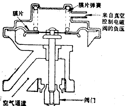
AAC valve
