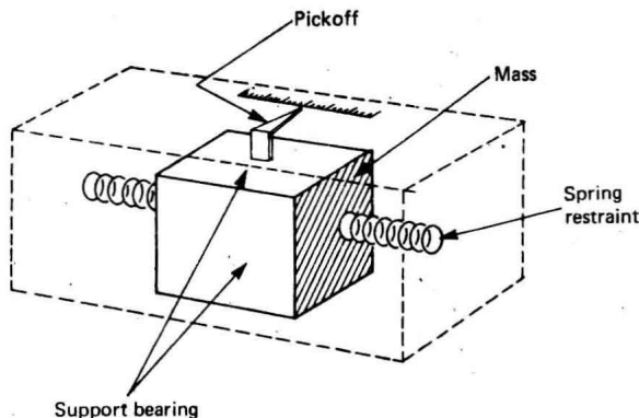
Fig. 1. Accelerometer based on a spring-restrained mass.
