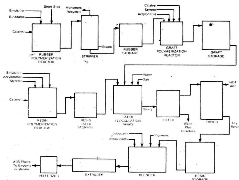
ABS manufacturing process. (Marbon Division, Borg-Warner Corporation)
