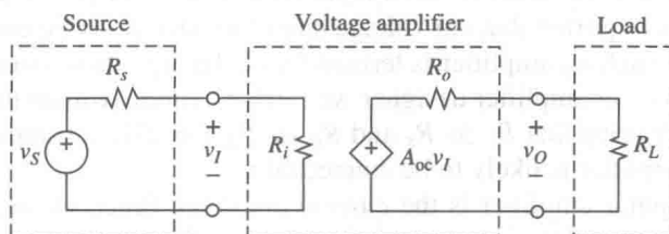
FIGURE 1.1 Voltage amplifier.
