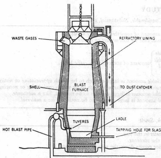
Cross-section of blast furnace
