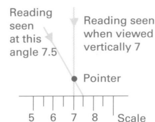
Figure 1.1 Parallax error
