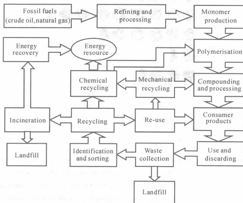
Figure 1.3 A “life guide”: following polymeric materials and products through cascades of uses from “cradle to grave”
