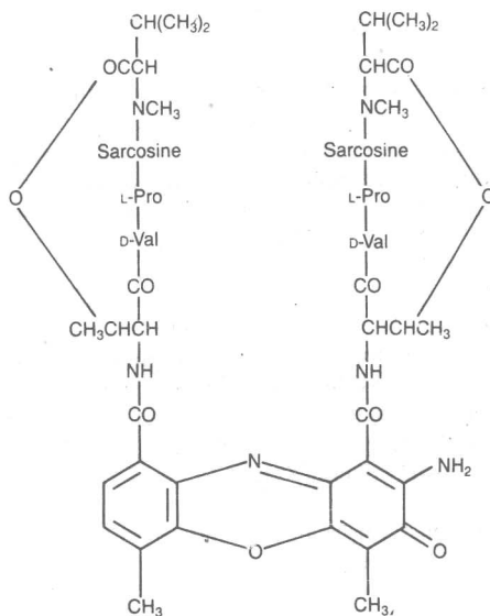
Actinomycin
