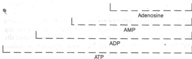
Adenosine nucleotides
