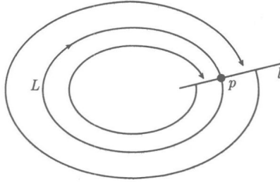
Figure 1.1.1 Behavior of a stable limit cycle
