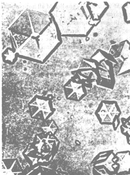
FIG. 1. Rhombohedral 2 Zn insulin crystals.
