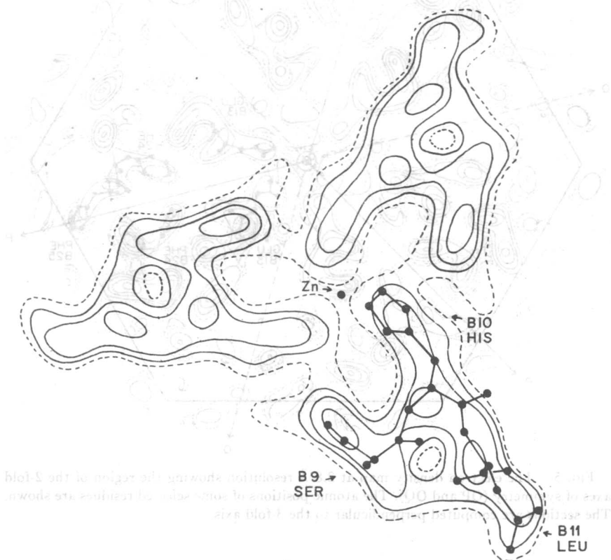
FIG. 4. The electron-density map at 2.8 Å resolution showing the appearances of residues B9, B10, and B11 of the insulin molecule. The section is taken perpendicular to the 3-fold axis. The atomic positions of one of the three equivalent groups are shown.
