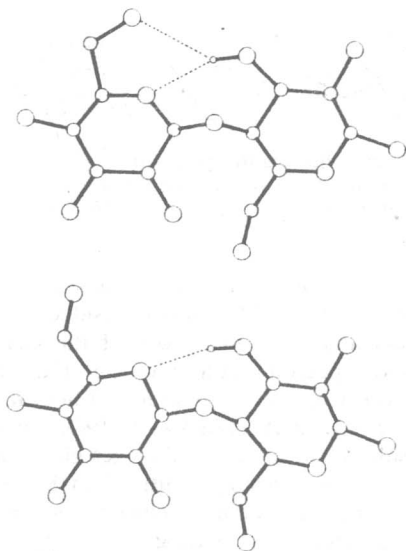
Fig. 2. Schematic representation of the anhydrocellobiose repeat units in the two ordered states, k_I (upper figure) and k_{II} (lower figure), based on the stable conformations of methyl \beta -cellobioside, with a bifurcated hydrogen bond (Ham & Williams, 1970), and cellobiose with one isolated hydrogen bond (Chu & Jeffrey, 1968), respectively. The computer-drawn figures were generated using molecular modelling (CHEMX, Chemical Design Ltd, Oxford, UK). Adapted from Atalla (1983).
