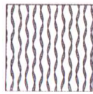
DNA
