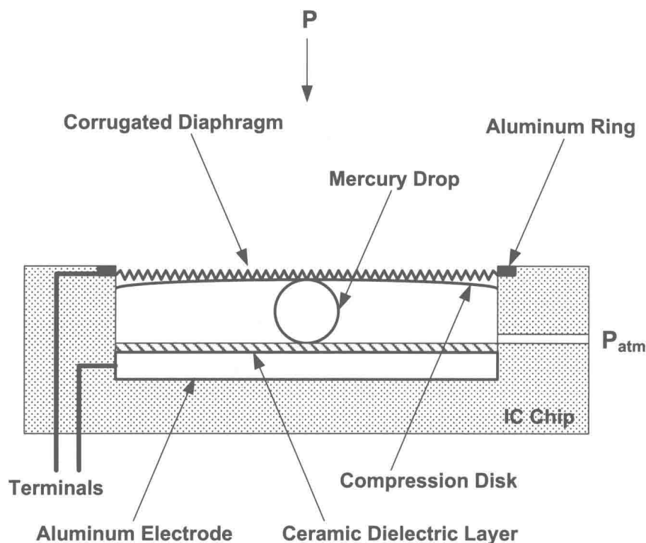
Figure 1.2: Mechanical structure of the sensor.
