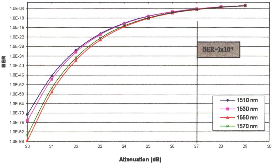
Figure 2. Effect of attenuation to BER performance for four different wavelengths for new additional signal.
