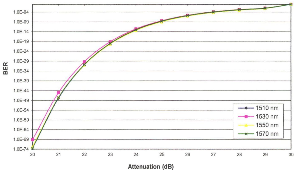
Figure 3. Effect of attenuation to BER performance for four different wavelengths for pass through operation.
