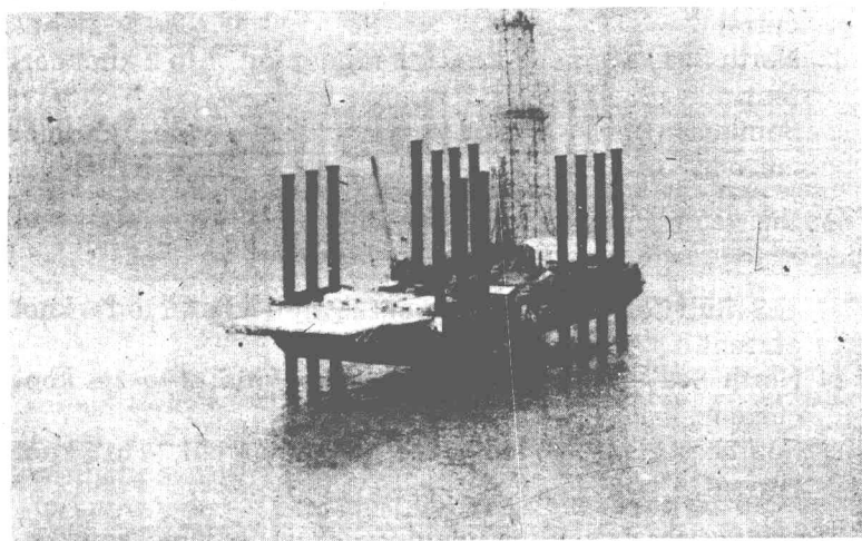
Fig. 1-5 Offshore's rig 52.
