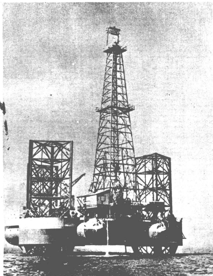
Fig. 1-6 LeTourneau's Scorpion.
