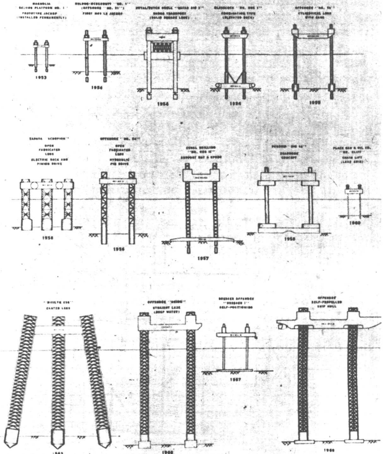
Fig. 1-3 Jack-up evolution.
