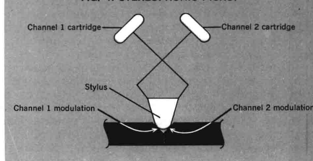
FIG. 4. STEREOPHONIC PICKUP
