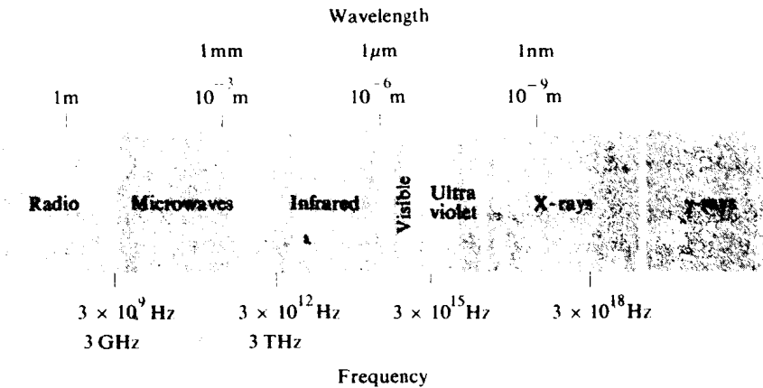
Fig. 2.1 The electromagnetic spectrum.
