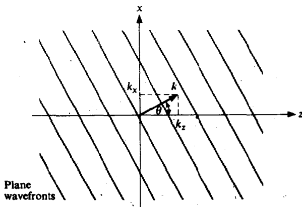
Fig. 2.4 Plane wave with propagation vector \mathbf{k} in the x - z plane (the y -axis is perpendicular to the page). The components of the propagation vector, k_x = |\mathbf{k}| \sin \theta and k_z = |\mathbf{k}| \cos \theta , are shown.
