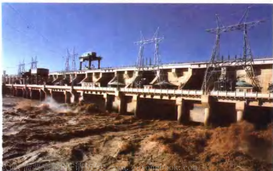
The Huanghe River Qingtongxia Key Water Control Project
