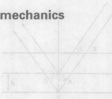
Figure 1.1 Scattering of two beams at angle \theta from two planes in a crystal spaced by d
